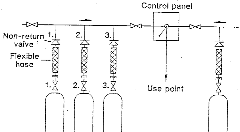
Figure 4 Manifold layout
