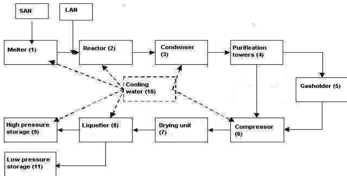
Figure 2: Scheme of nitrous oxide production
