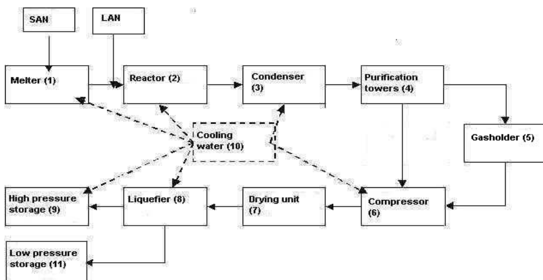
Figure 2: Scheme of nitrous oxide production
