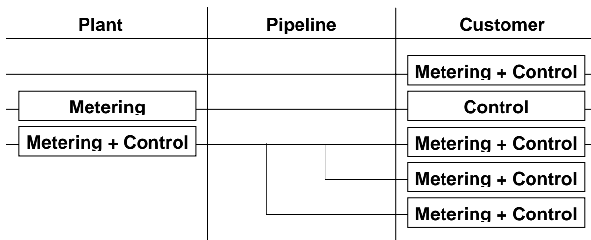
Diagram 1 : Typical transmission and distribution piping systems
