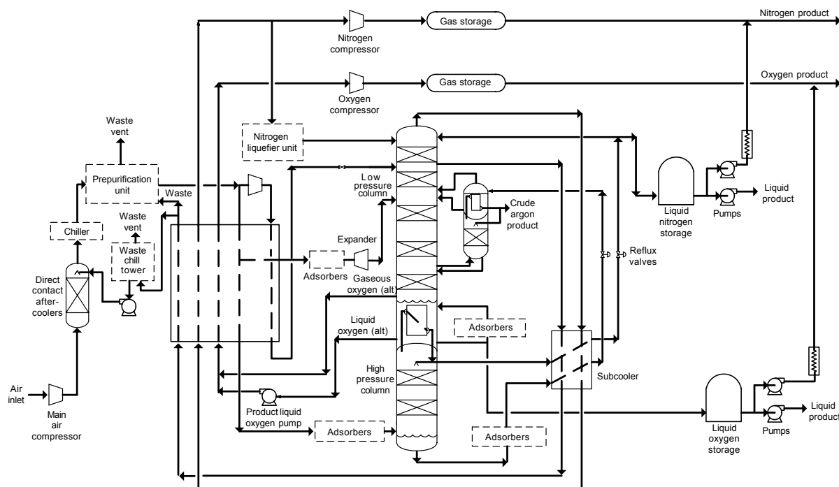
Oxygen has the highest boiling point of the three main components and is taken from the bottom of the LP column. Nitrogen is taken from the top of the LP or HP columns. An argon-rich stream can be withdrawn from the middle of the LP column and refined to a pure product in other distillation columns. The product streams are warmed to ambient temperature against incoming air in the main heat exchanger to recover the refrigeration. It is also possible to remove the products from the distillation system as liquid if sufficient refrigeration is available. Producing large quantities of liquid products requires extra refrigeration, often supplied by a nitrogen liquefier unit. Liquid may be stored for pipeline back-up or merchant sales.
