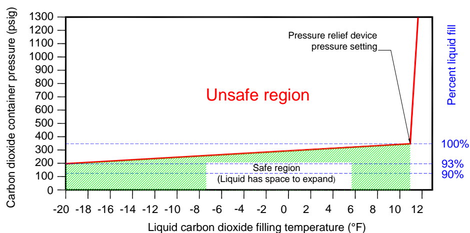
Figure 4—Safe filling volumes for 350 psig carbon dioxide containers
