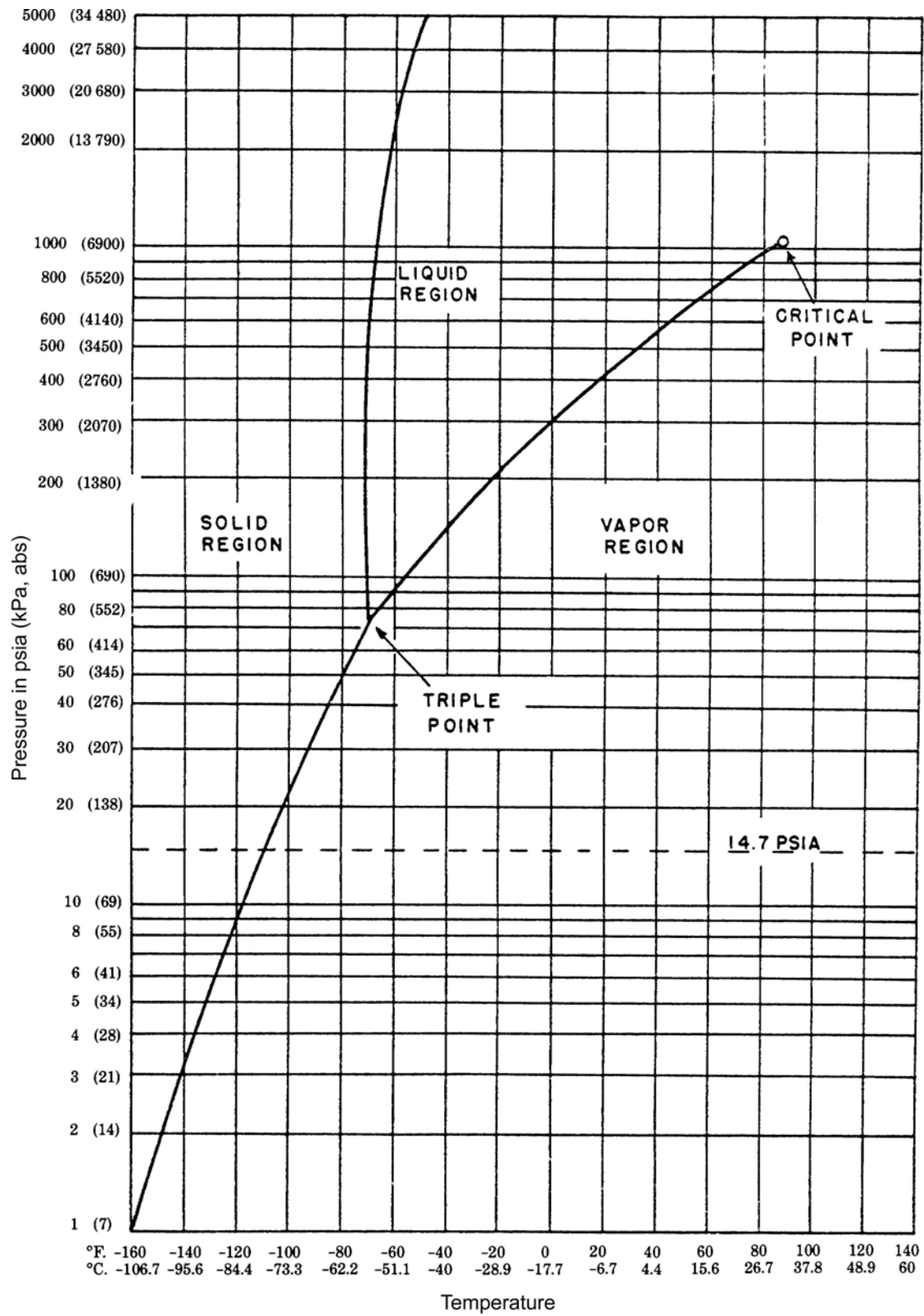
Figure 1—Carbon dioxide phase diagram
