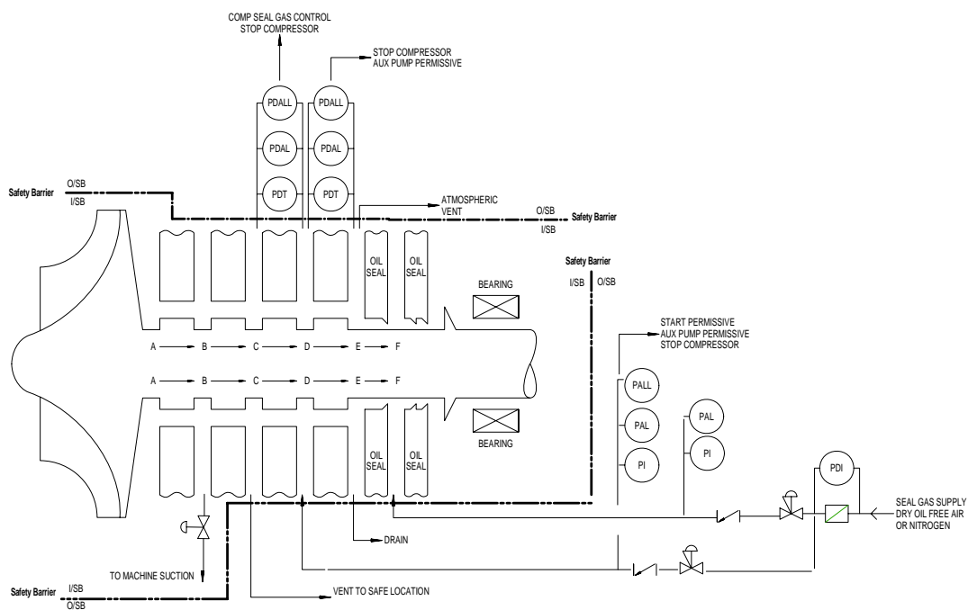
Figure 3.1 Single shaft Seal Gas Supply Schematic Diagram
