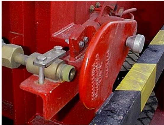
Figure B-1: Tow-away incident prevention device blocking the coupling when activated
