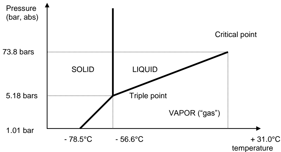
Diagram 1: section of CO 2 pressure-temperature diagram
