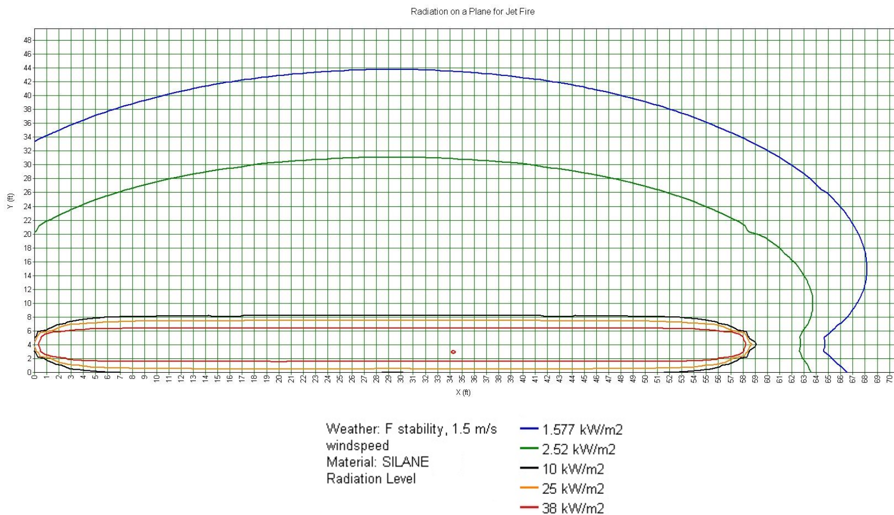
Figure D-23—Thermal radiation for package without pressure relief device and in use—pigtail release with no restrictive flow orifice
