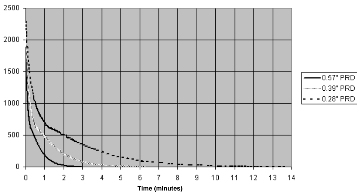
Figure D-10—Pressure relief device release time for a ton tank (450 L container)
