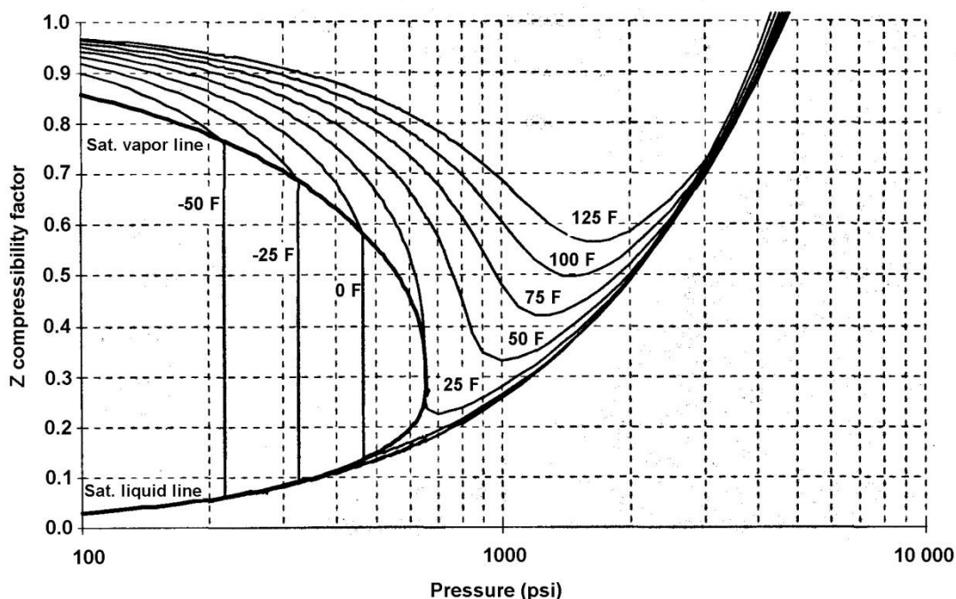
Figure B-1—Silane compressability
