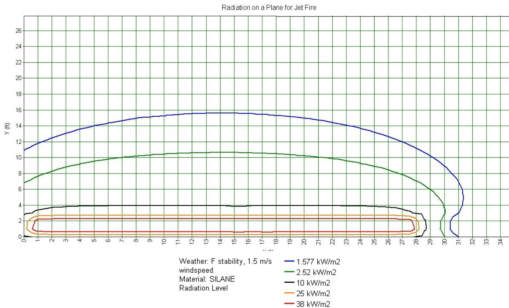
Figure D-22—Thermal radiation for package without pressure relief device and in use—pigtail release with 0.060 in restrictive flow orifice
