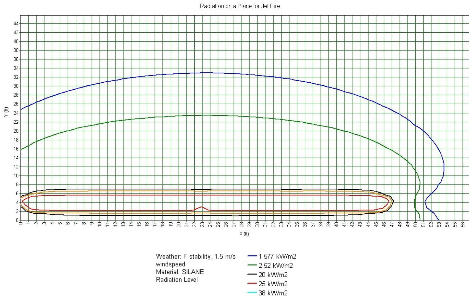
Figure D-21—Thermal radiation for package without pressure relief device and in use—pigtail release with 0.125 in restrictive flow orifice
