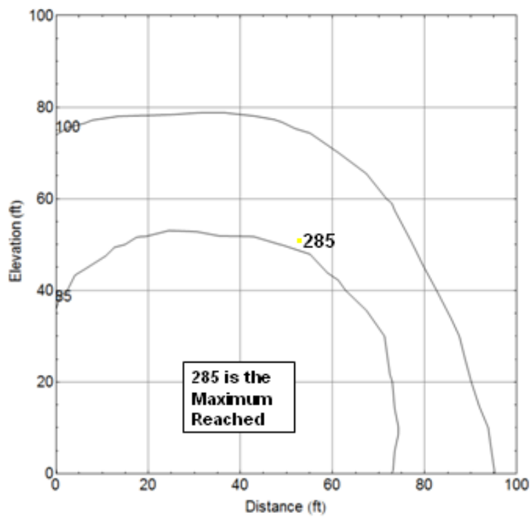
Figure D-8—Thermal dose for ton tank with 0.28 in pressure relief device, 100% flow for use
