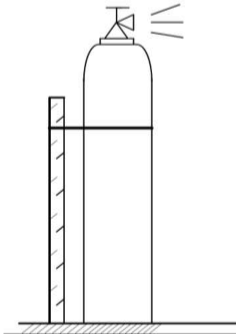
Figure 7—Method 4A: Direct discharge from container valve
